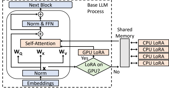
Figure 7: Illustration of coordinated LoRA computation on GPU and CPU per transformer block’s attention layer.
