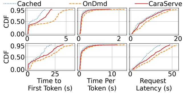
Figure 15: Evaluation on Llama2-13B (Top) and Llama2-70B (Bottom) models with RPS = 6, rank = 64 .
