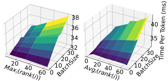
Figure 4: The varying decoding latency of batching heterogeneous LoRA adapters. Left: The performance of Punica’s BGMV [1] is determined by the batch size and the maximum rank . Right: The performance of S-LoRA’s MBGMV [23] depends on the batch size and the average rank in the batch.
